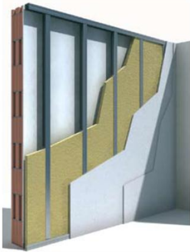
■ Controparete W625
